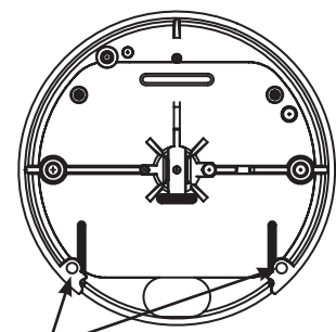
Insert Springs & Pins Figure 8
